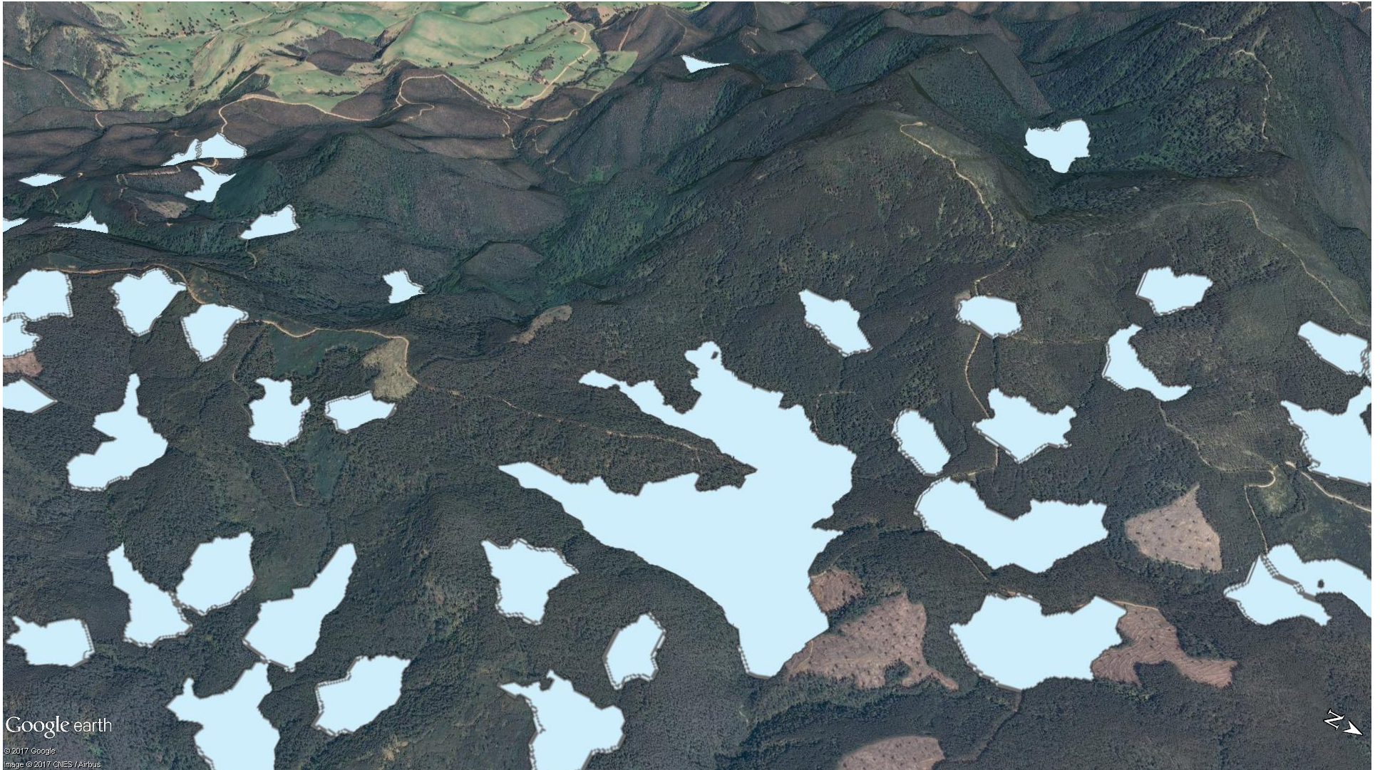
Figure 13: Potential PHES upper reservoir sites near Nunniong (Victoria) The site in the centre has a very good water to rock ratio.
