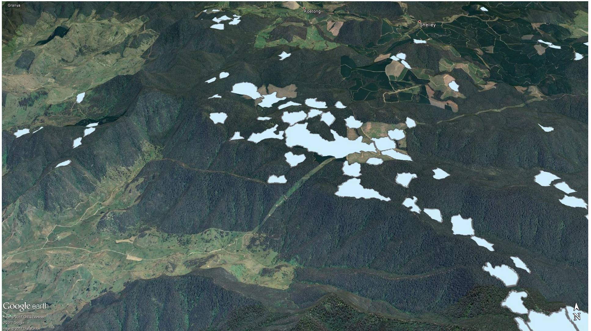
Figure 14: Potential PHES upper reservoir sites near the Tallangatta Valley (Victoria) The easement corridor for the 330 kV transmission line can be seen in this image.
